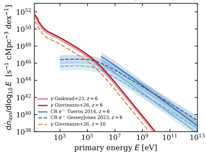
(b) differential ionizing emissivity
