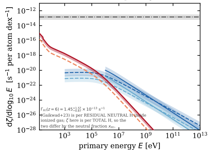
(c) ionization rate per target atom
