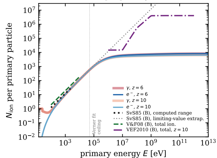
(a) ionizations per primary, full cascade
